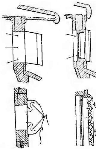
Figs. 4319-20, SMALL DUPLEX DEFLECTOR.
